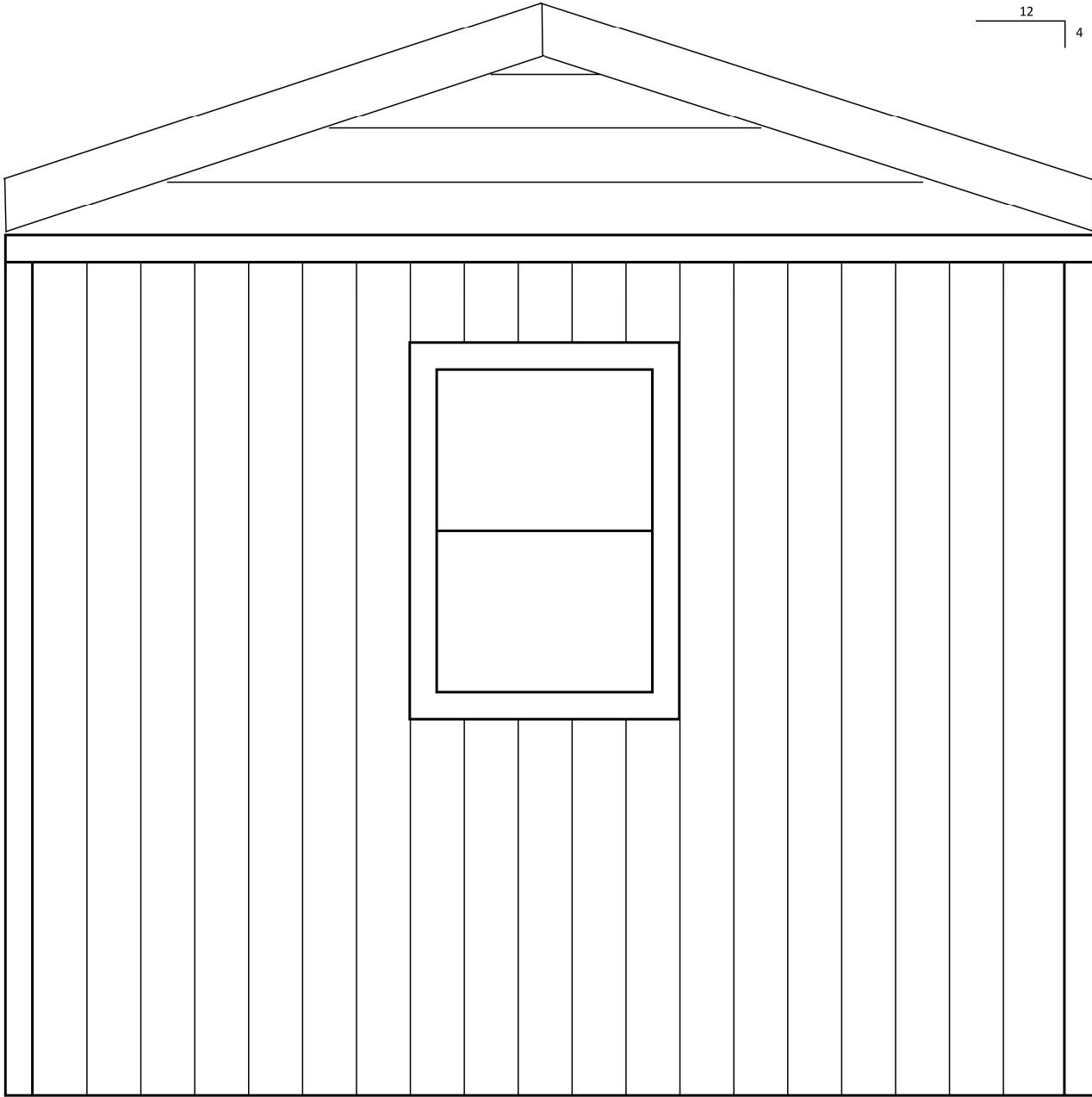
REAR ELEVATION
