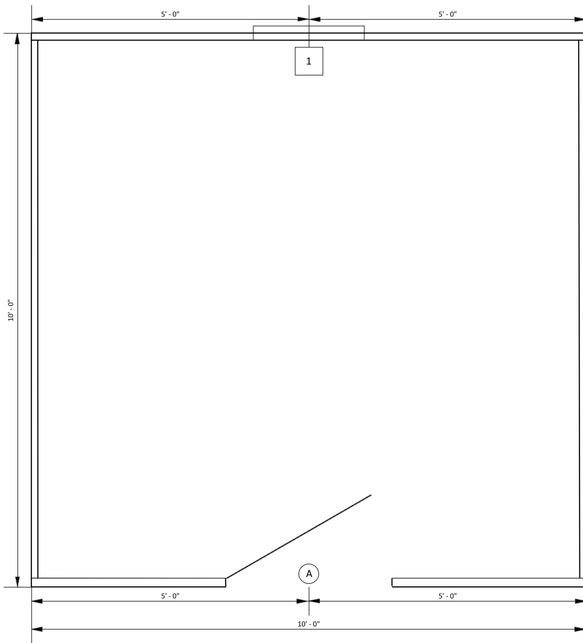
FLOOR PLAN
